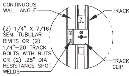
DETAIL F
