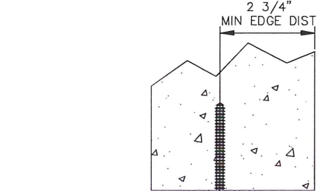
MOUNTING TO STEEL DETAIL
